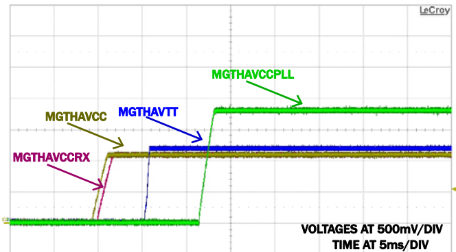
FIGURE 3. START-UP SEQUENCE
